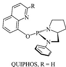
Figure 2. Well-known P *, N -bidentate diamidophosphite ligand QUIPHOS
