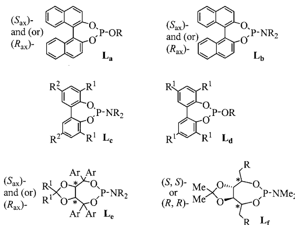
Figure 1. Some well-known efficient P -monodentate chiral phosphites and phosphoramidites
